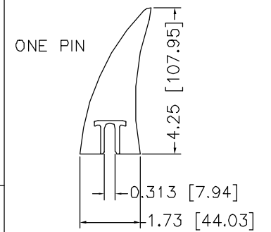
MODEL "GSS" BOLTS INTO FRAME
